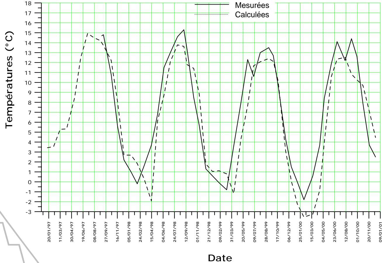
Comparison between measured and calculated temperatures – BLOC 3
